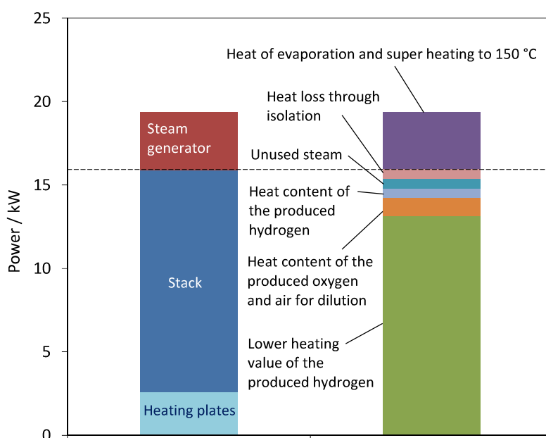
Figure 2. Energy demand of the Jülich rSOC system for electrolysis.
